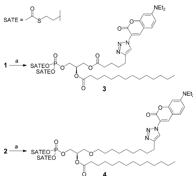
Scheme 1. Synthesis of the fluorescent phosphatidic acid derivatives 3 and 4 : a) 3-azido-7-(diethylamino)coumarin, CuSO 4 , sodium ascorbate, EtOH/H 2 O (1:1).
