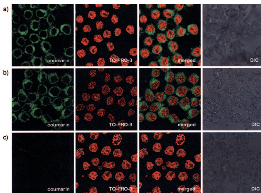
Figure 1. Fluorescence microscopic images of fixed RAW macrophages treated with the PA derivatives 1 or 2 for 1 h and with 3-azido-7-(diethylamino)coumarin, CuSO 4 , sodium ascorbate, and TBTA for 30 min. a) Cells treated with 1 and the nuclear marker TO-PRO-3 iodide. b) Cells treated with 2 and the nuclear marker TO-PRO-3 iodide. c) Negative control cells treated with 3-azido-7-(diethylamino)coumarin, CuSO 4 , sodium ascorbate, and TBTA only. DIC = differential interference contrast.
