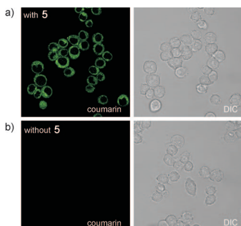
Figure 2. Fluorescence microscopic images of living RAW macrophages. a) Cells treated with 5 for 1 h and 3-azido-7-(diethylamino)-coumarin for 3 h. b) Negative control cells treated with 3-azido-7-(diethylamino)coumarin for 3 h only.
